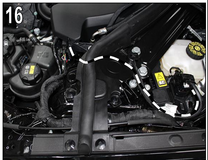
Fig. 16 with MHEV Lay AC Schnitzer wiring harness, in the area of the spring dome on the left, below the rubber seal. If necessary, remove rubber seal.
